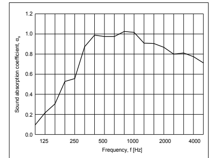
Sound Test Figure 3: Installation: 45 mm air gap behind the panel. Closed frame around the edge.
