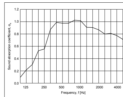
Sound Test Figure 3: Installation: 45 mm air gap behind the panel. Closed frame around the edge.
